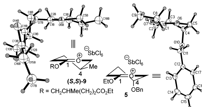
Figure 1. Crystal structures of dioxocarbenium ions 5 and 9 .
